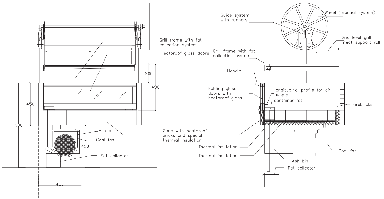
CROSS SECTION
